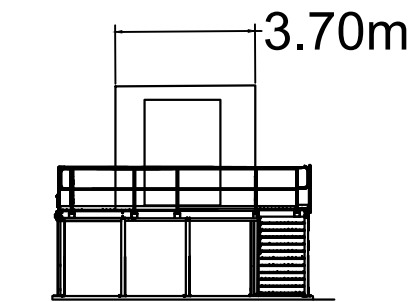
SIDE ELEVATION
