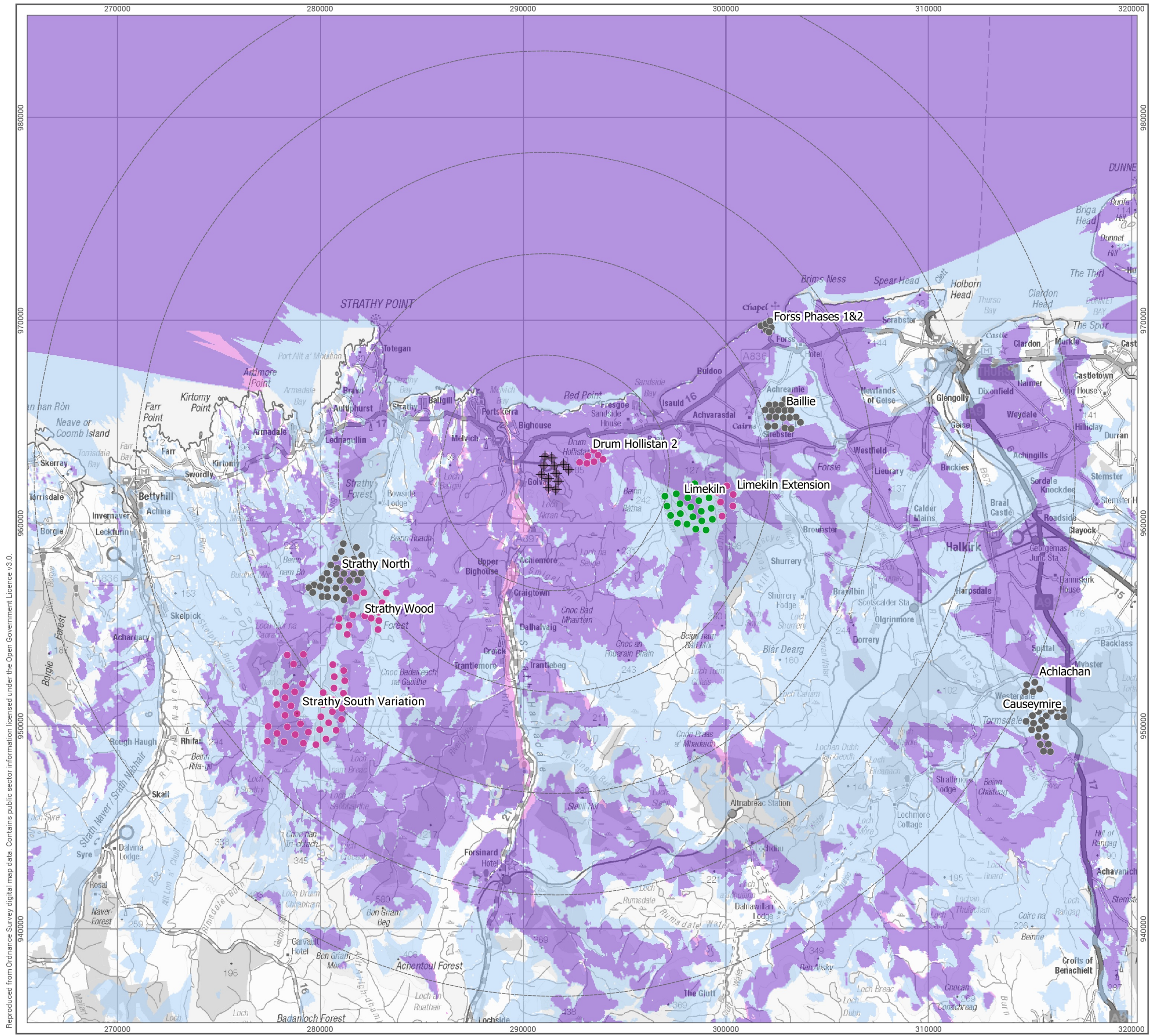
Cumulative ZTV with Existing, Consented and 'In planning' Wind Farms Figure 6.11
