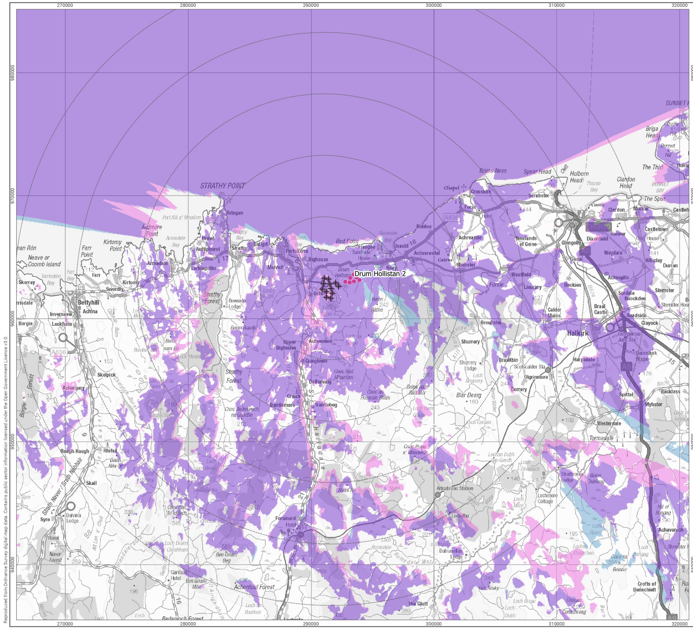
Cumulative ZTV with Drum Hollistan 2 Figure 6.11a Ackron Wind Farm
