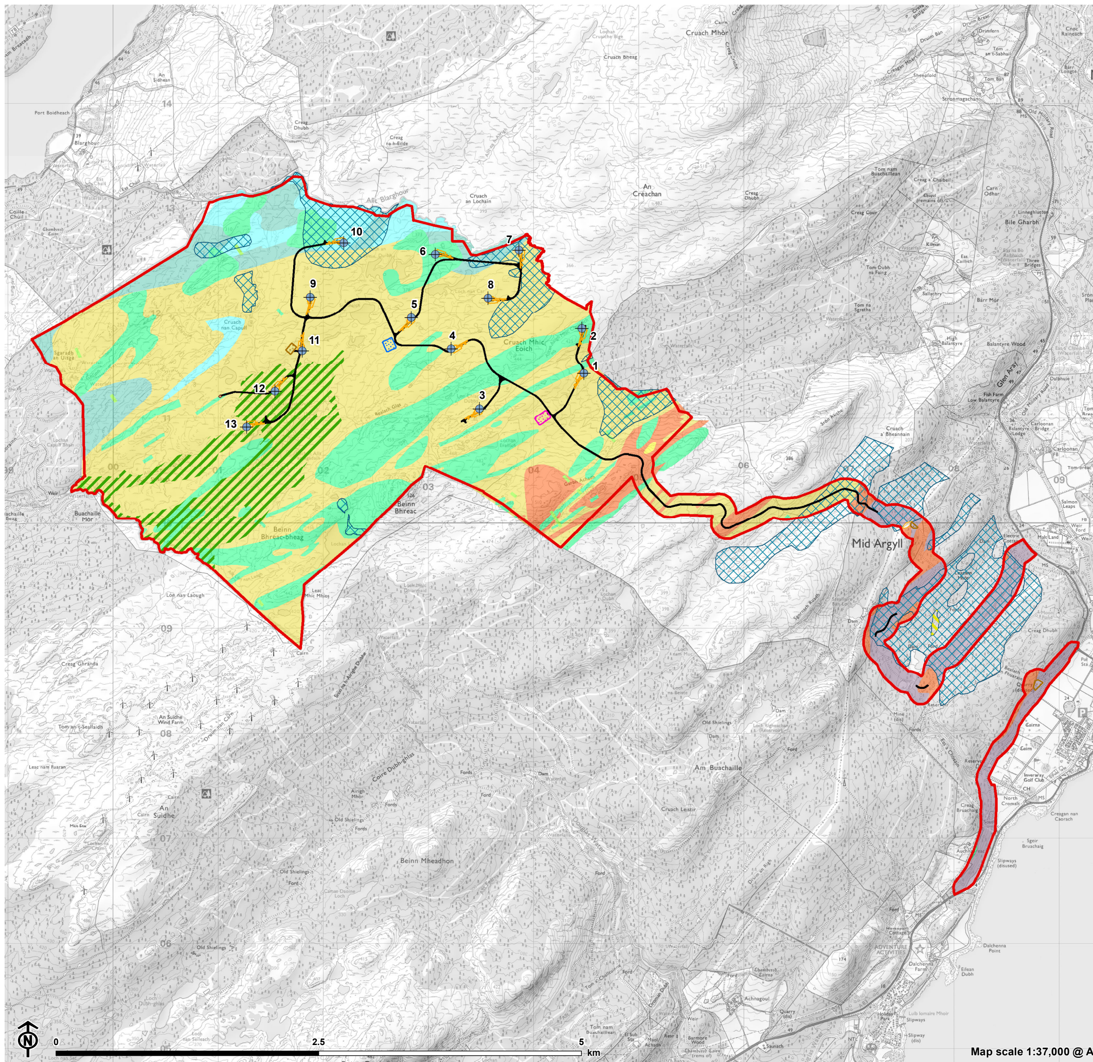
Figure 7.4: Superficial and Bedrock Geology
