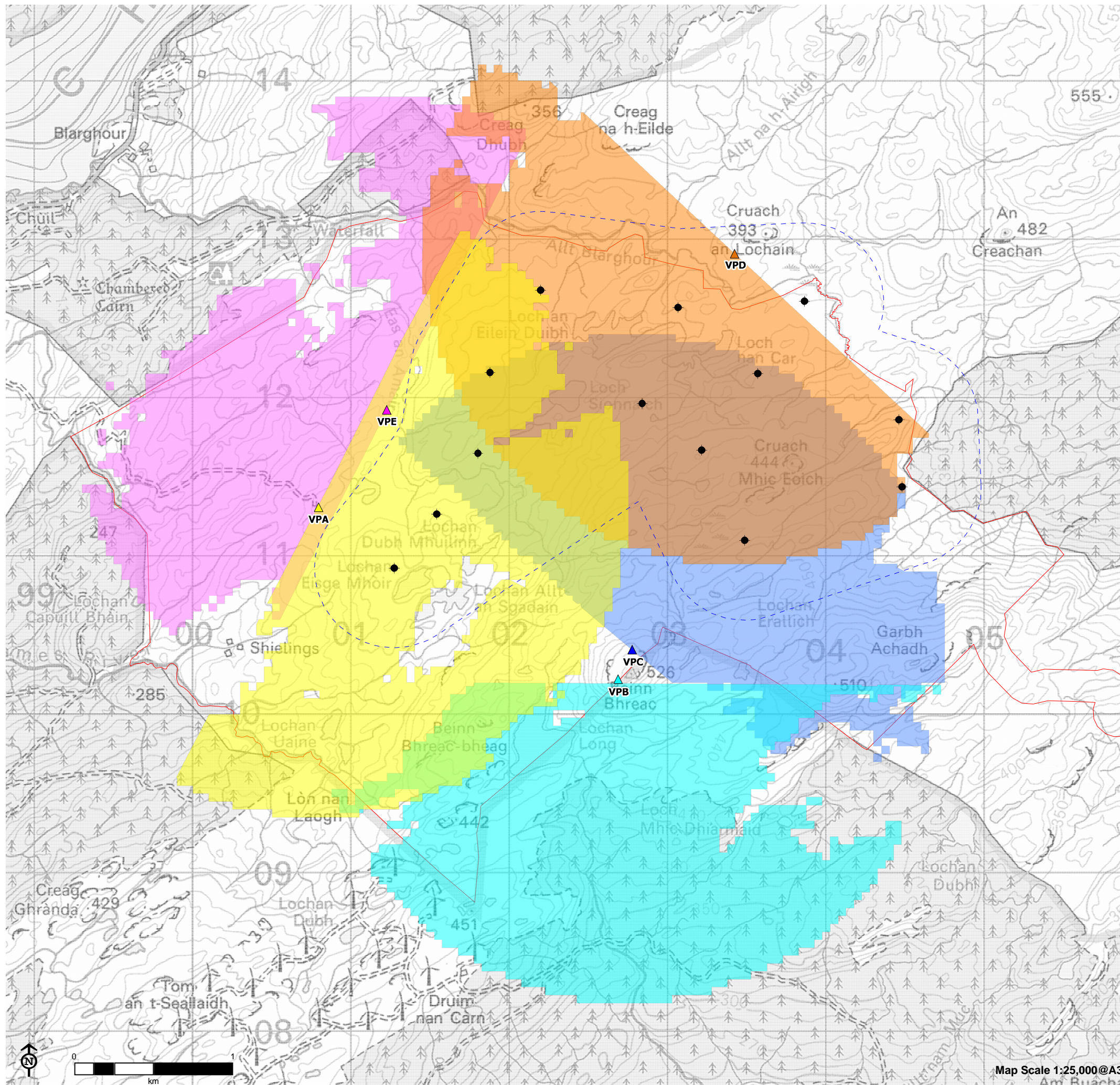
Figure 9.3: Vantage Point (VP) Survey Plan
