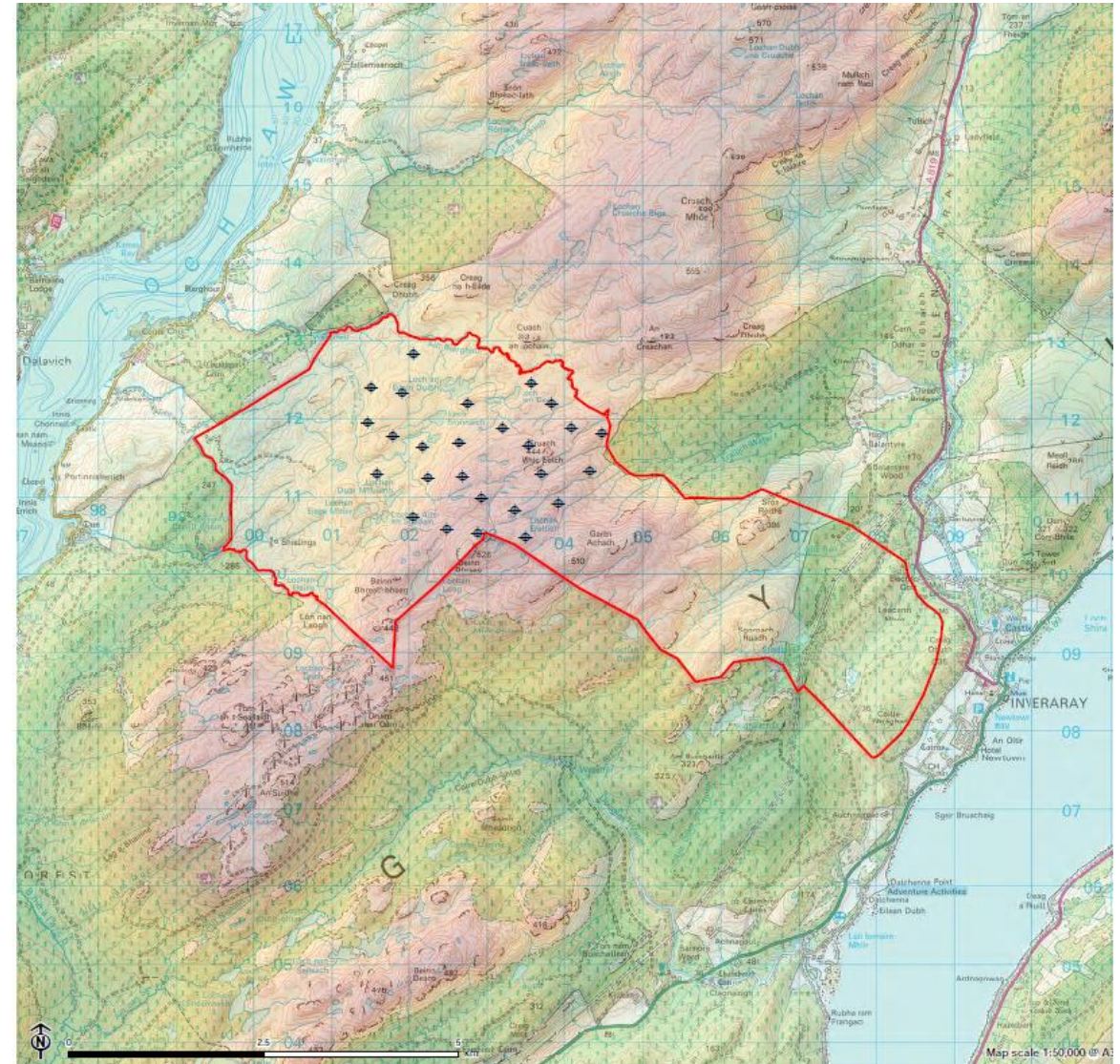
Figure 3.1: Proposed Turbine Layout
