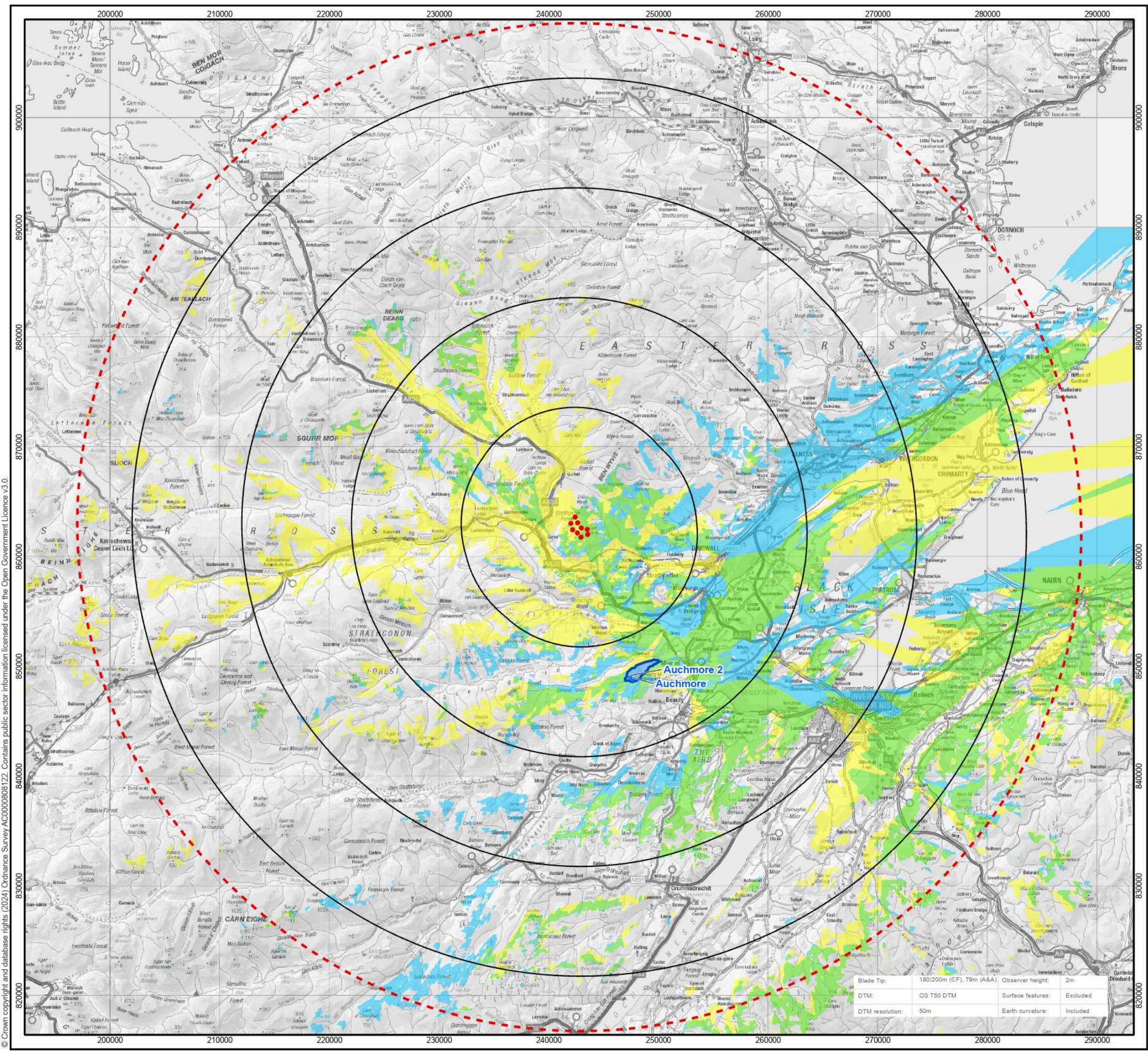
Figure 7.15e Cumulative ZTV - Auchmore and Auchmore 2 (45km Radius) Carn Farna Wind Farm Environmental Impact Assessment Report
