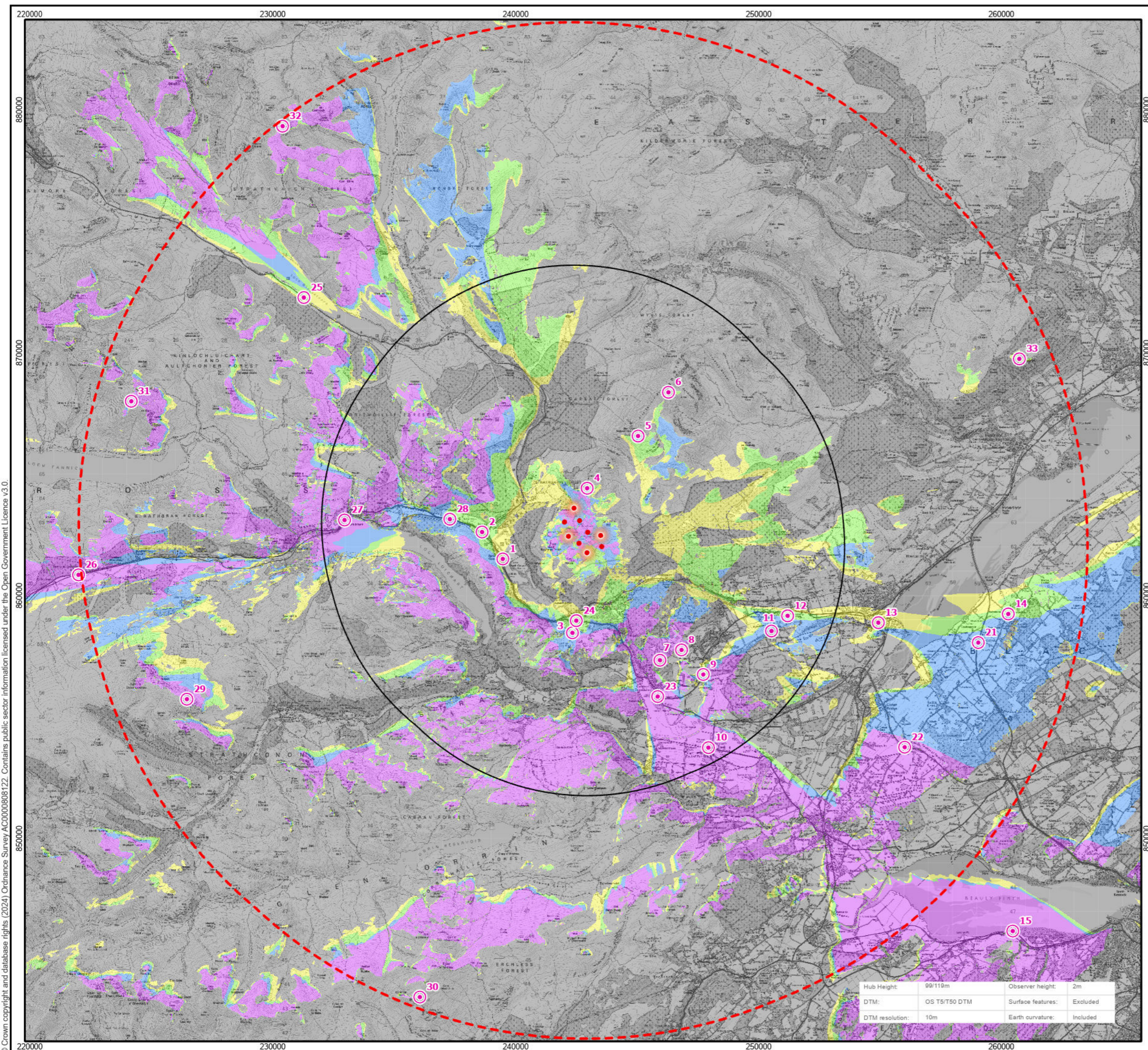
Figure 7.9b Turbine Lighting ZTV Carn Ferna Wind Farm Environmental Impact Assessment Report
