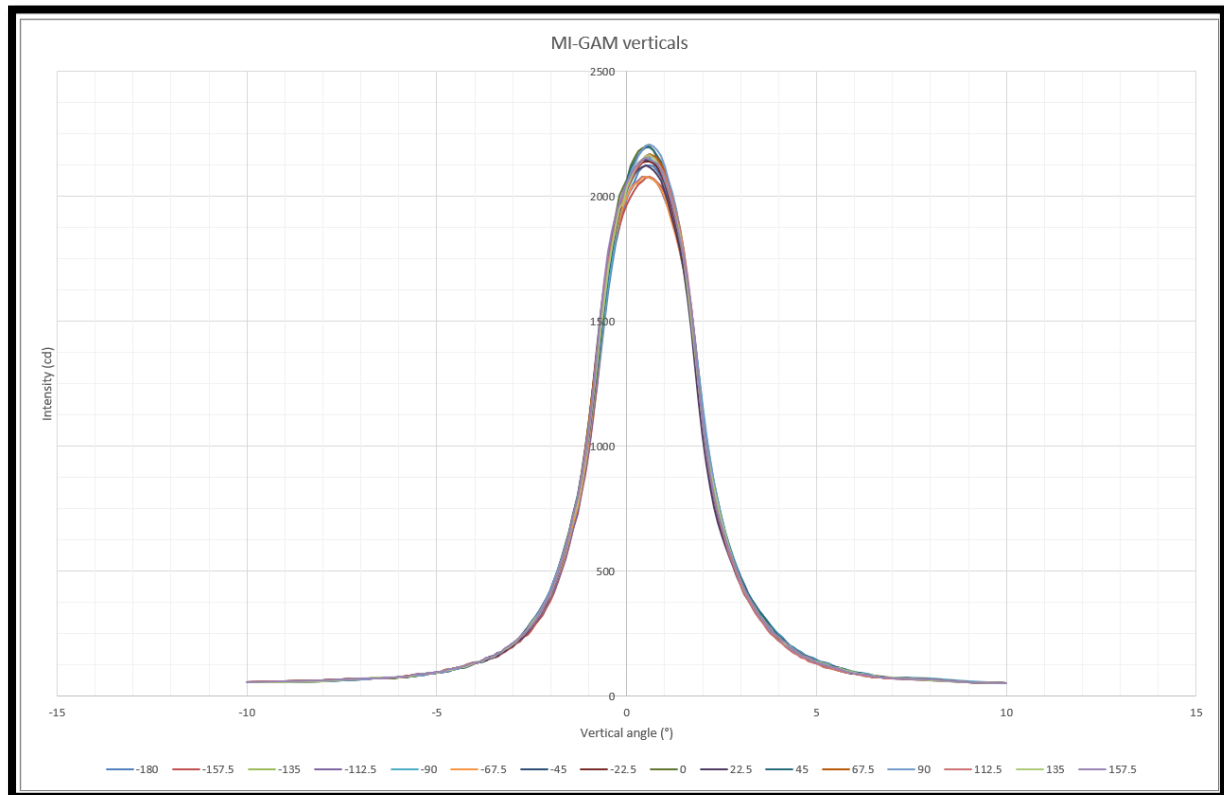
Figure 9 CEL-WT-MIC Light Measurement Results
