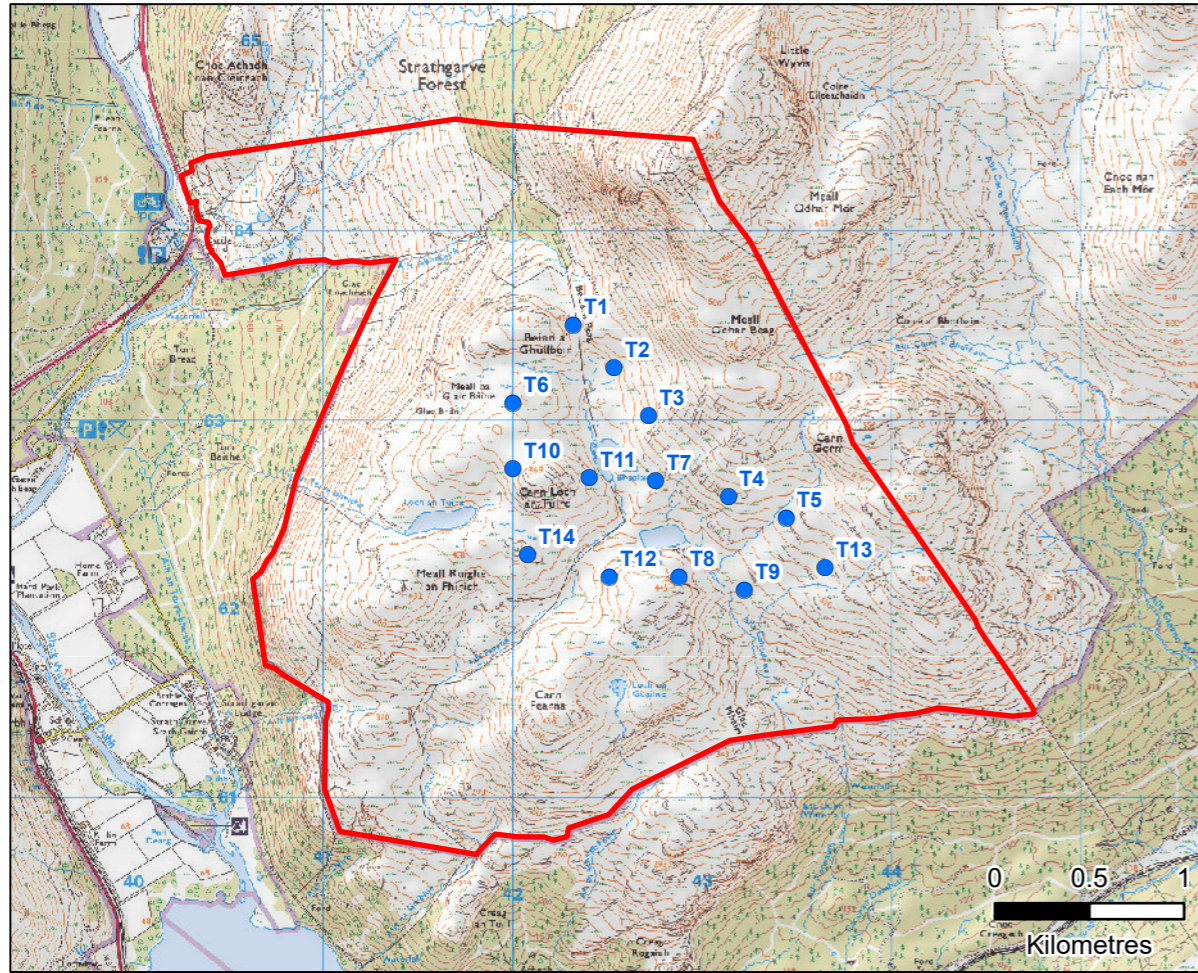
Carn Gorm Wind Farm Layout 2013
