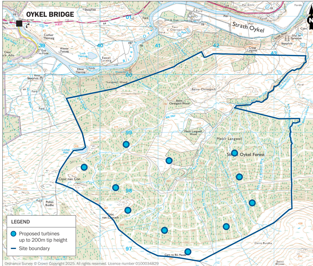
Plan showing Coille Beith Wind Farm layout.
