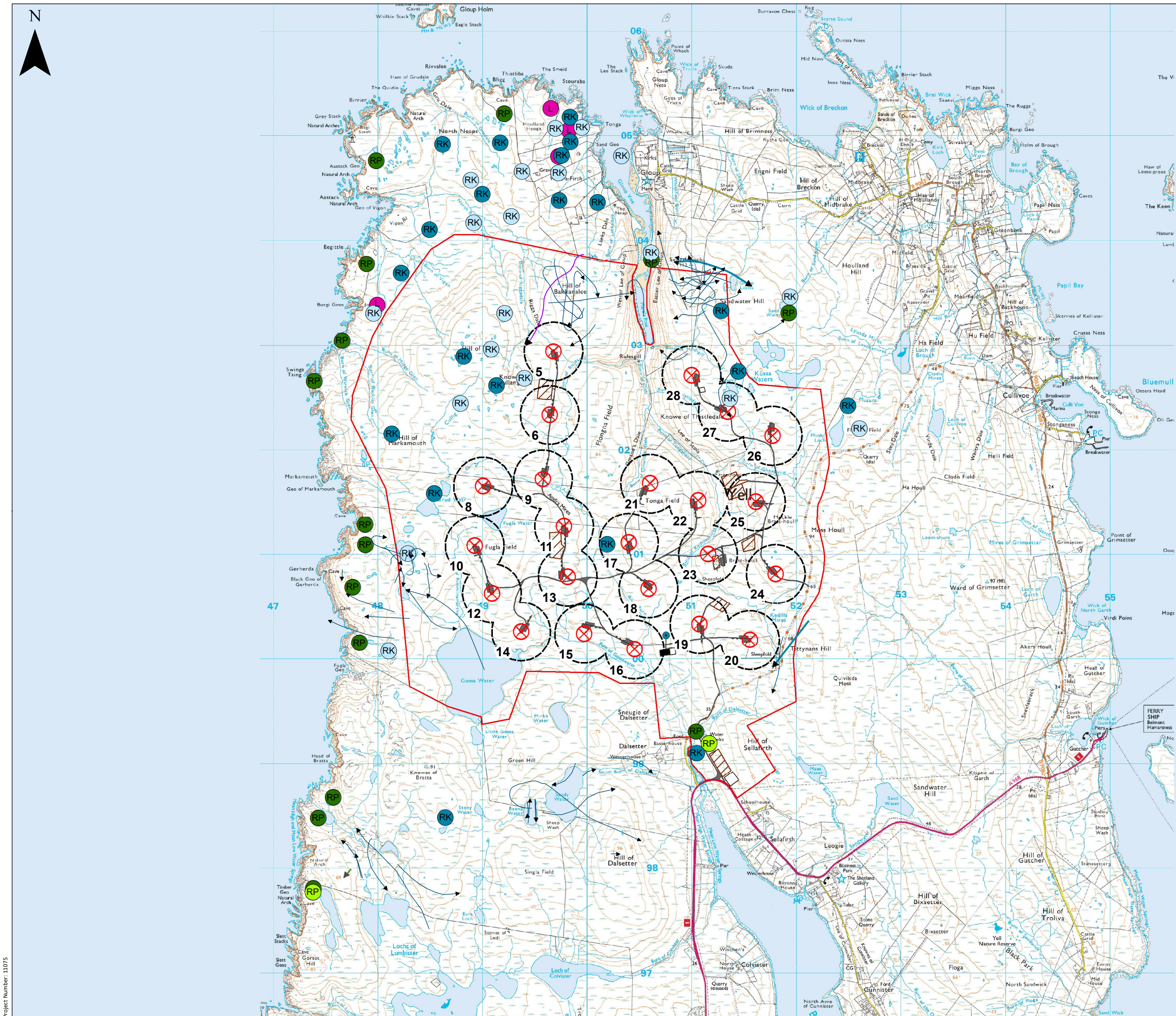
Energy Isles Wind Farm Supplementary Environmental Information Figure 6.15 Lapwing, Ringed Plover and Redshank territories and flights
