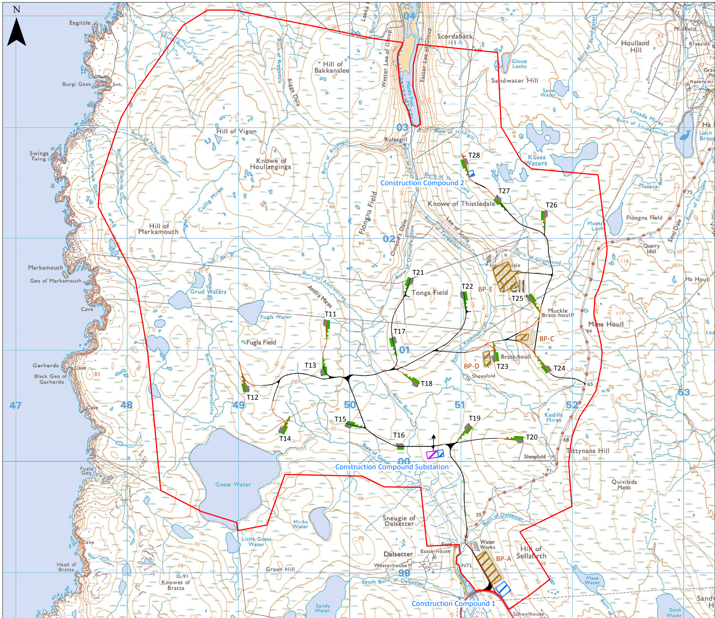
Energy Isles Wind Farm Supplementary Environmental Information 2 Figure 1.1 Site Layout Plan - 2021 Layout
