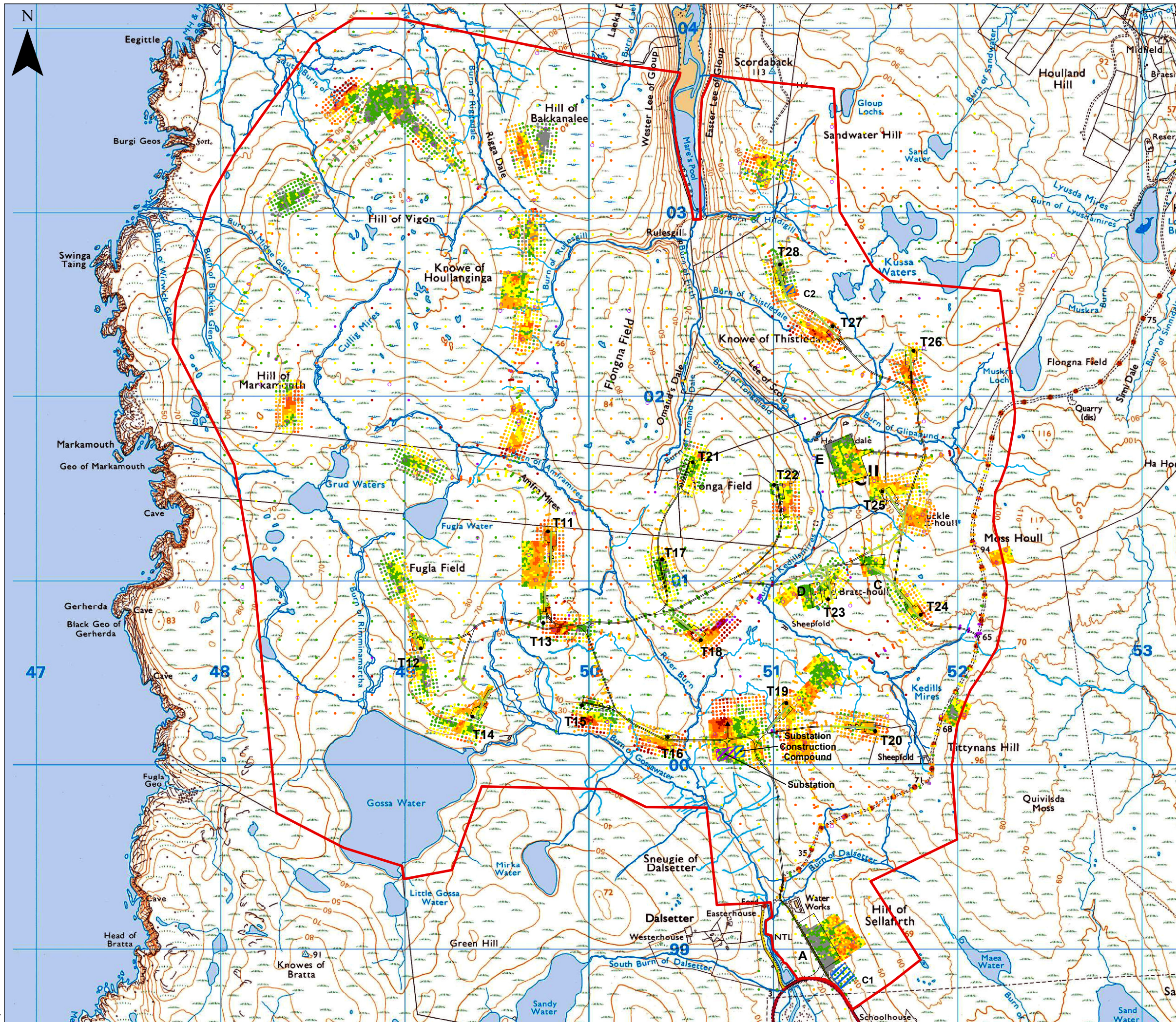
Energy Isles Wind Farm Supplementary Environmental Information 2 Figure 10.8 Depth of Penetration at Probing Locations
