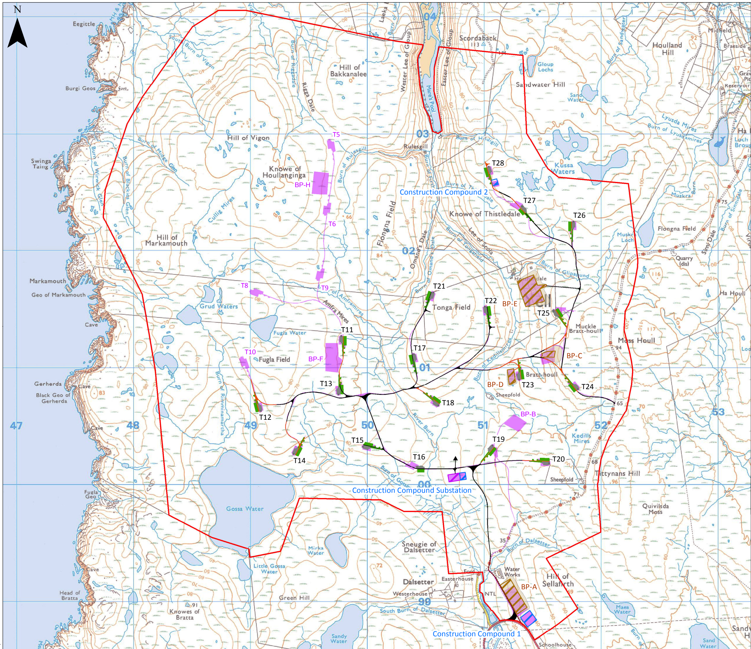
Energy Isles Wind Farm Supplementary Environmental Information 2 Figure 3.2 2020 Layout to 2021 Layout Comparison
