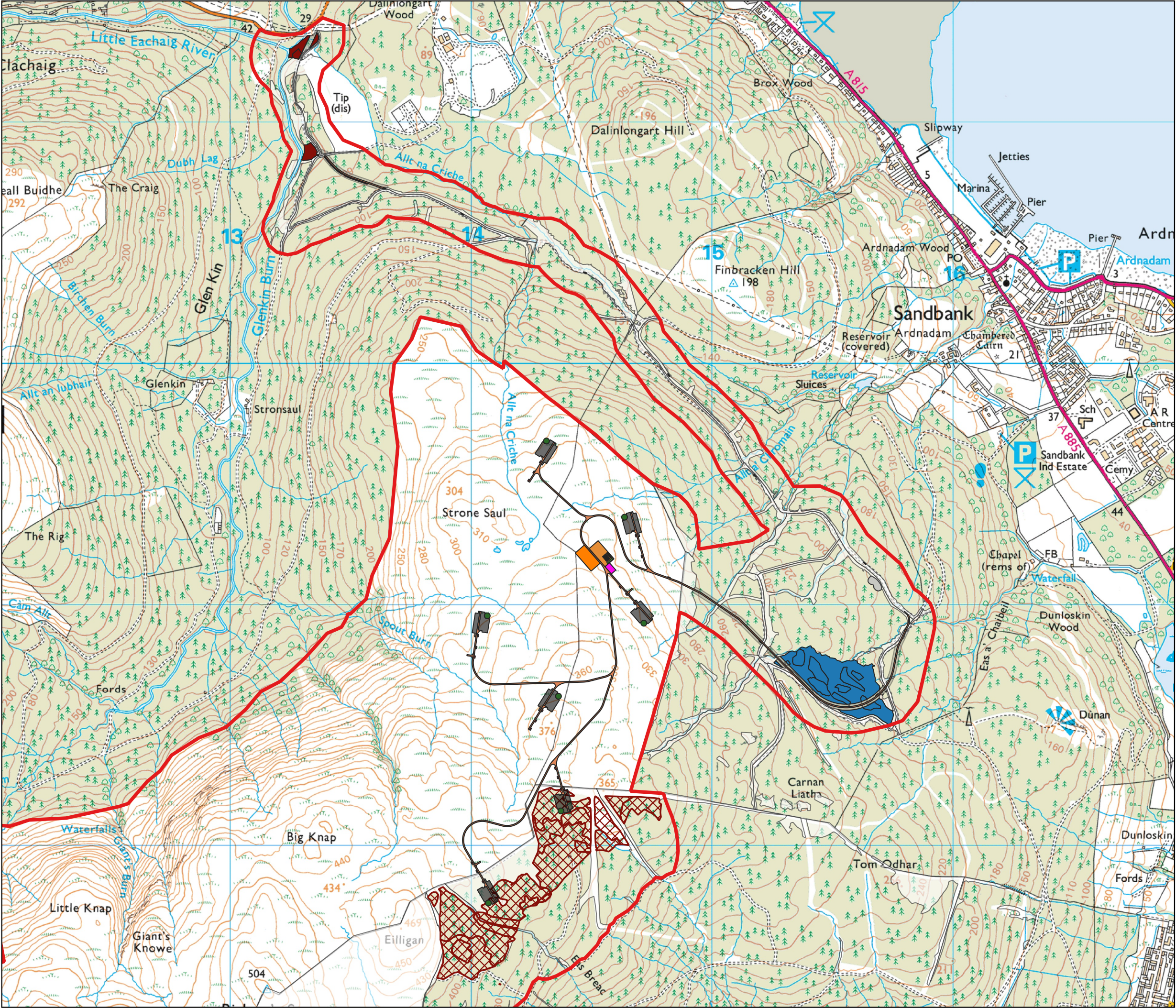
Figure 12.4 Replanting Plan Giant's Burn Wind Farm EIA Report
