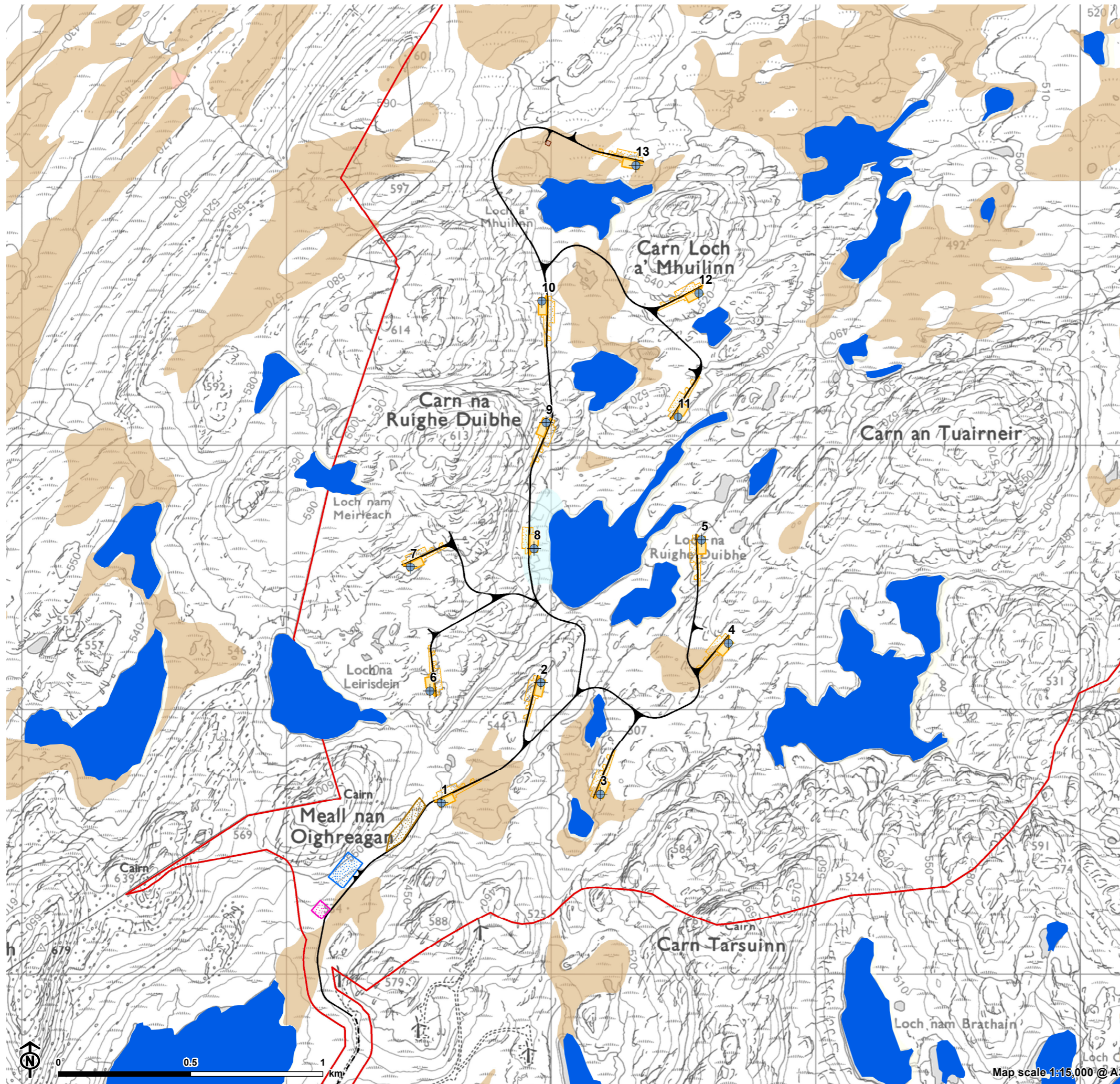
Figure 7.4: Superficial Geology
