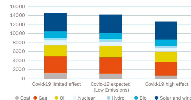
Global demand for primary energy in 2050 with various long-term effects of the COVID-19 epidemic (Mtoe)
