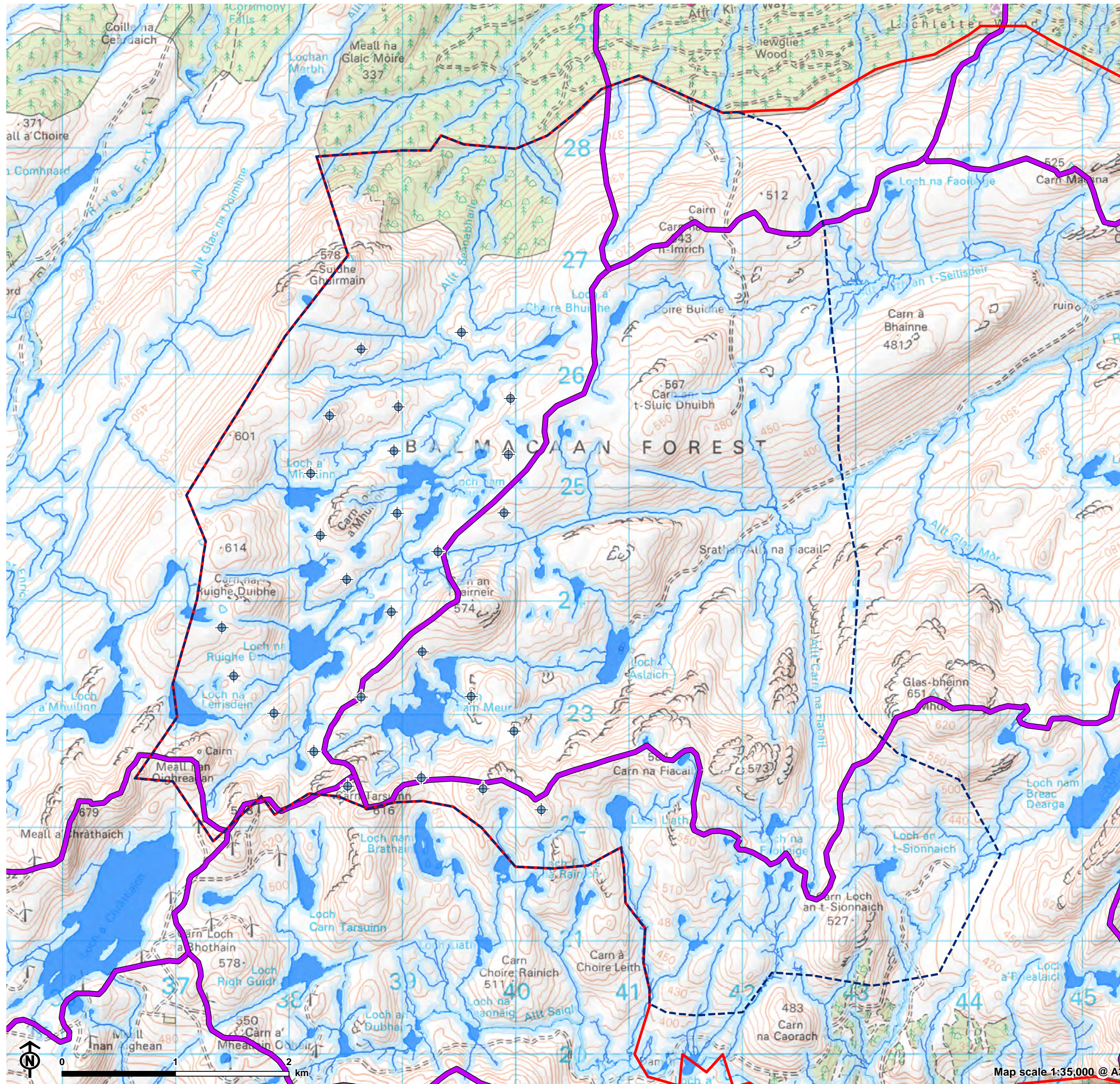
Figure 6.1: Hydrology Features
