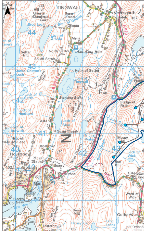
Plan showing Mossy Hill Wind Farm redesign proposal layout.
