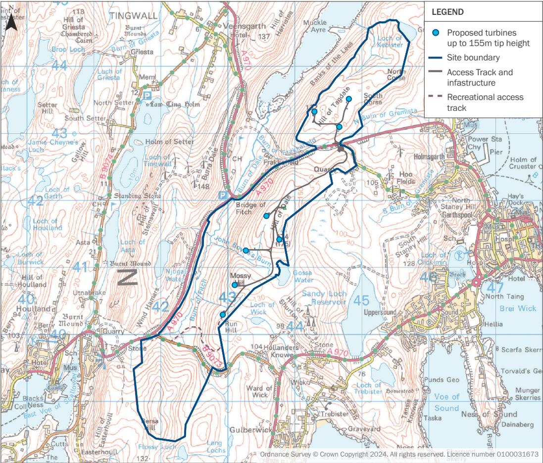
Plan showing Mossy Hill Wind Farm redesign proposal layout.
