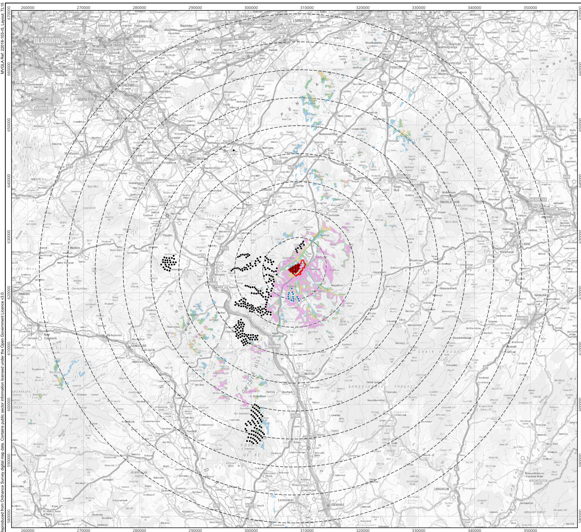
Figure 7.3 Zone of Theoretical Visibility at Turbine Hub Height (45km) Oliver Forest Wind Farm Environmental Impact Assessment Report
