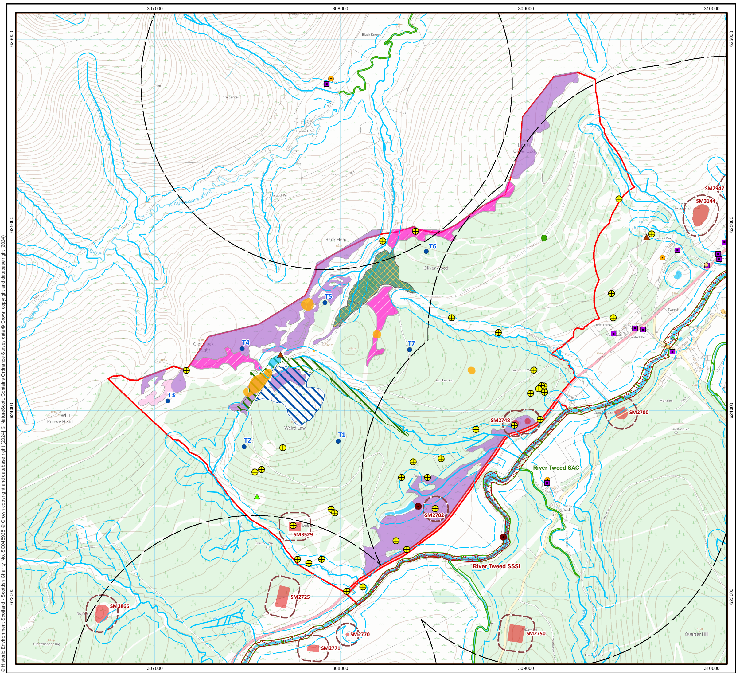
Figure 2.2 On-Site Constraints Oliver Forest Wind Farm Environmental Impact Assessment Report
