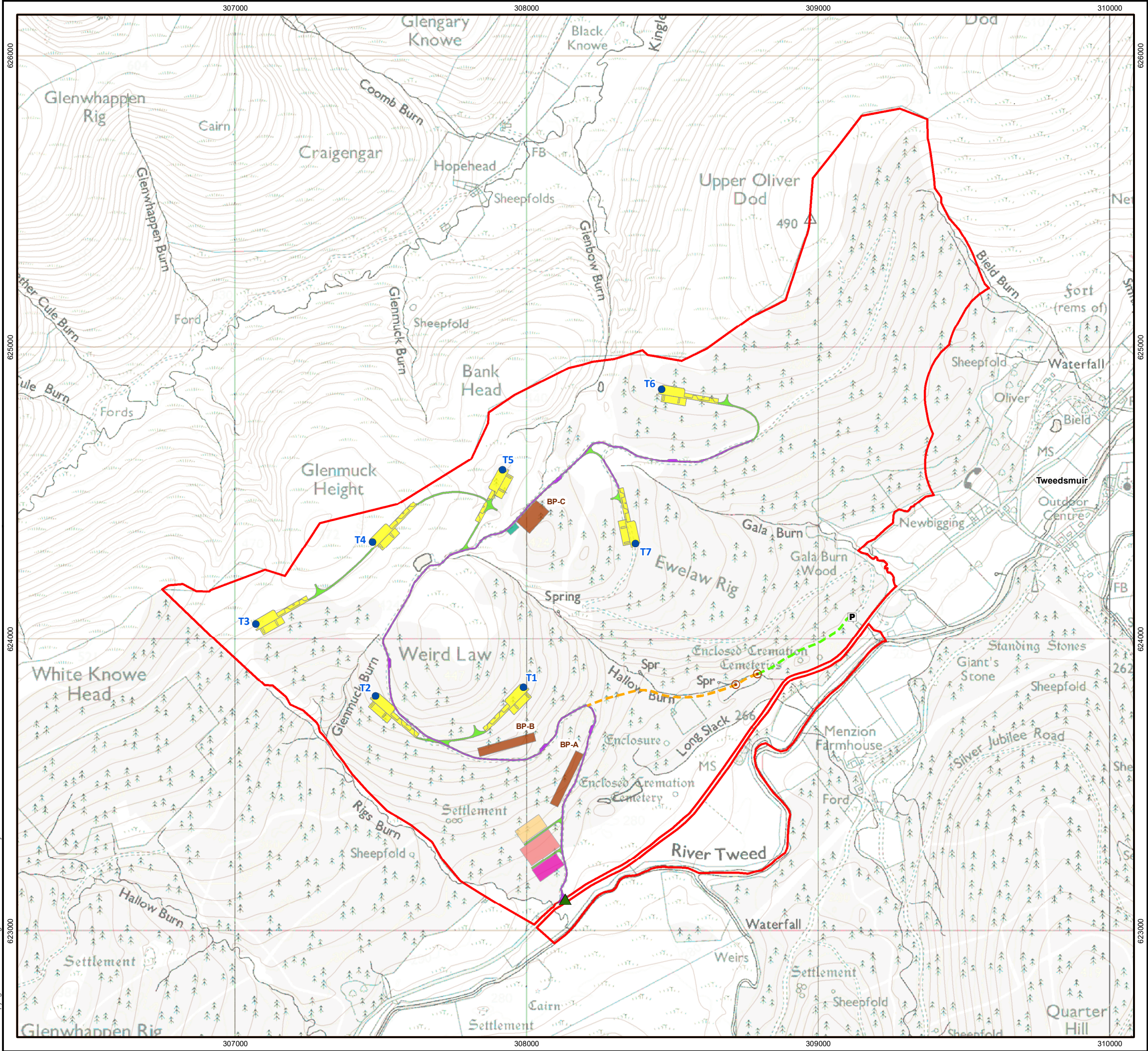
Figure 10.2.2 Site Layout Oliver Forest Wind Farm Environmental Impact Assessment Report
