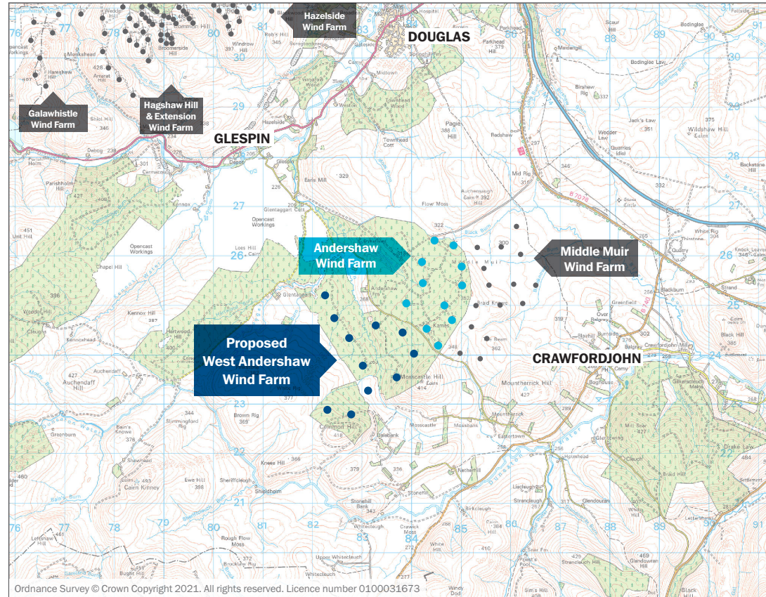
Plan showing proposed West Andershaw Wind Farm and current operational wind farms.
